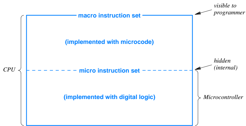
Figure 8.3 Illustration of a CPU implemented with a microcontroller. The macro instruction set that the CPU provides is implemented with microcode.
