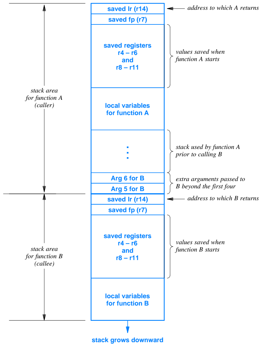
Figure 27.3 Layout of items on the run-time stack just after function A calls function B with six arguments.
