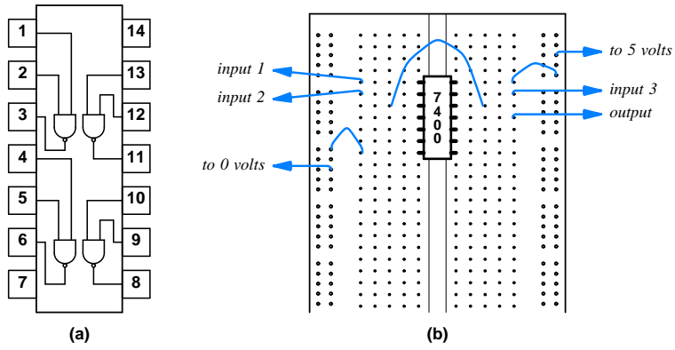
Figure 24.2 Illustrations of (a) the internal connections on a 7400 chip, and (b) part of a breadboard with blue lines indicating wires connecting a 7400 chip. Using a set of sockets to connect power and ground wires allows additional connections to be added.
