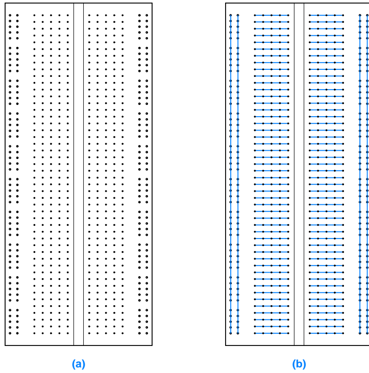
Figure 24.1 (a) Illustration of a breadboard with sockets into which wires can be inserted, and (b) blue lines showing the electrical connections among the sockets.
