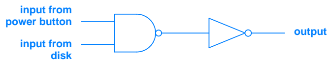
Figure 2.7 Illustration of gate interconnection. The output from one logic gate can connect directly to the input of another gate.
