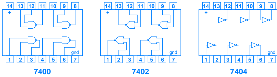
Figure 2.13 Illustration of the pin connections on three commercially available integrated circuits that implement logic gates.
