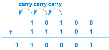
Figure 2.10 Example of binary addition using carry bits.
