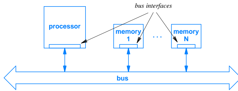
Figure 15.7 Physical interconnections of a processor and memory using a memory bus. A controller circuit in each device handles the details of bus access.
