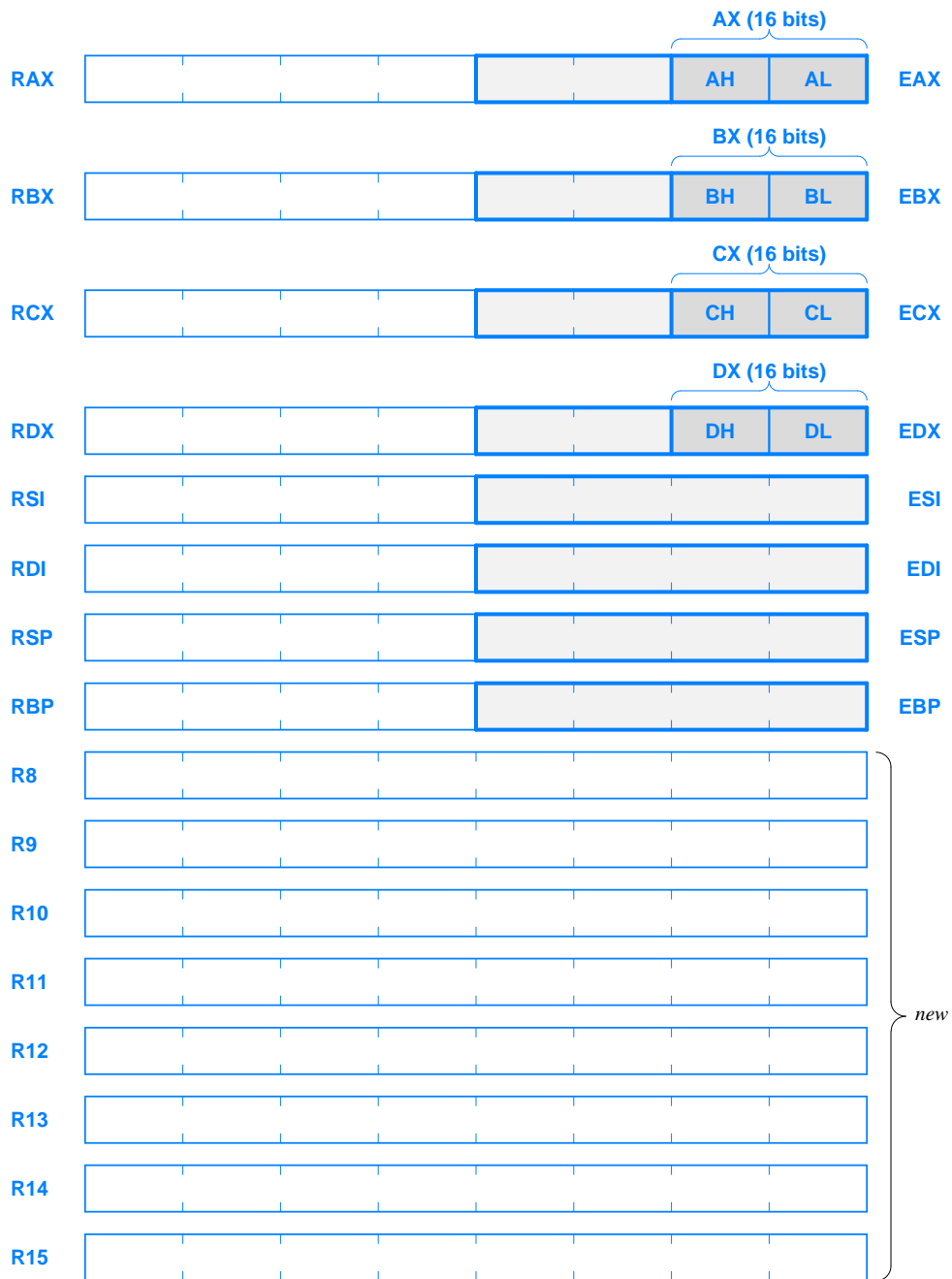
Figure 26.16 General-purpose registers in the x64 architecture.
