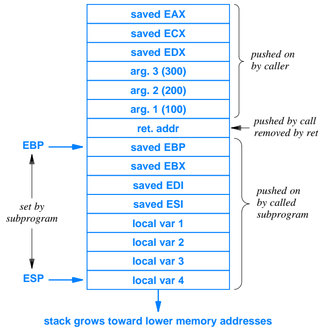
Figure 26.15 Illustration of the run-time stack after a subprogram has been called with three arguments and the subprogram has reserved space for four local variables.
