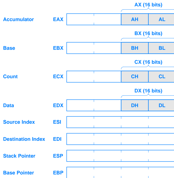
Figure 26.1 The eight general-purpose registers on an x86 processor, their historical purpose, and the names used to reference a register and the subparts.
