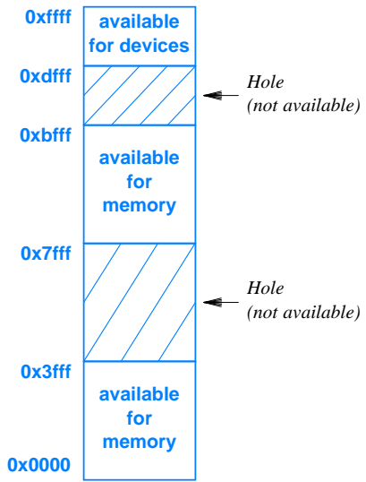
Figure 15.14 One possible address map for a sixteen-bit bus. Two areas are available for memory, and one area is available for devices.
