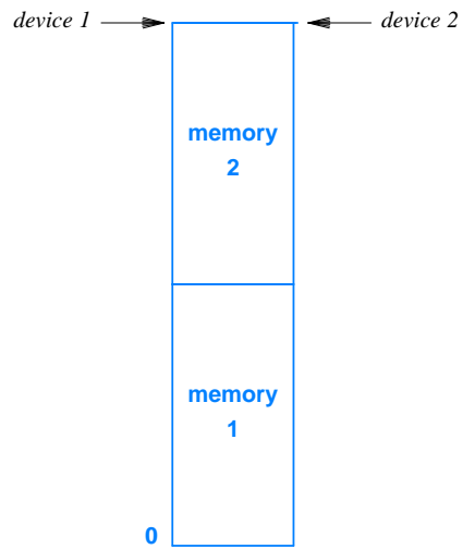
Figure 15.13 Illustration of the address space that results from the address assignments in Figure 15.12. The amount of space taken by each device (twelve bytes) is insignificant compared to the amount of space taken by each memory (1 Mbyte).
