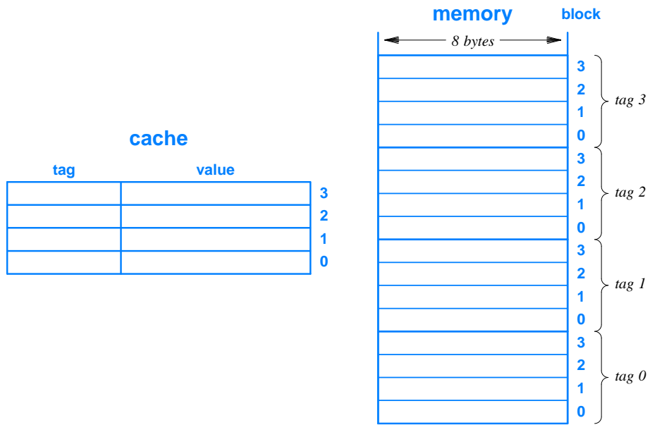
Figure 12.8 An example memory cache with space for four blocks and a memory divided into conceptual blocks of 8 bytes. Each group of four blocks in memory is assigned a unique tag.
