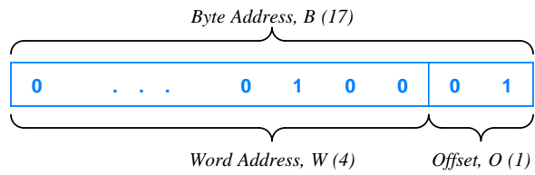
Figure 11.8 An example of a mapping from byte address 17 to word address 4 and offset 1. Using a power of two for the number of bytes per word avoids arithmetic calculations.
